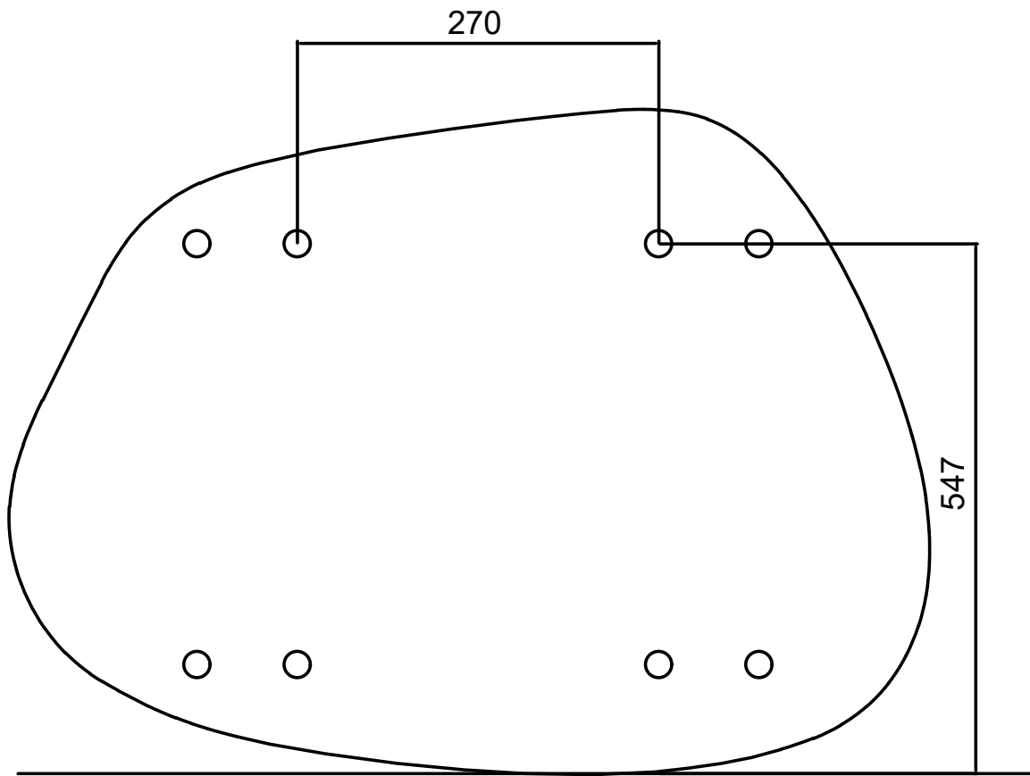
Horizontal Mirror Mounting Reference point
